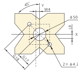
Front boring(fixed or plug-in circuit breaker)(мм)
